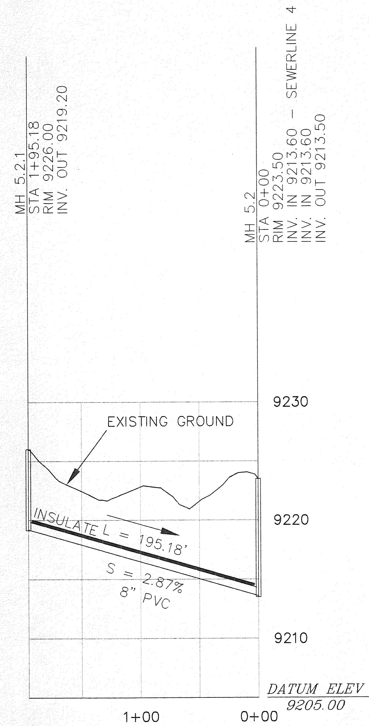
SEWER MAIN #5 SCALE: HORIZONTAL - 1" = 50' VERTICAL - 1" = 5'
