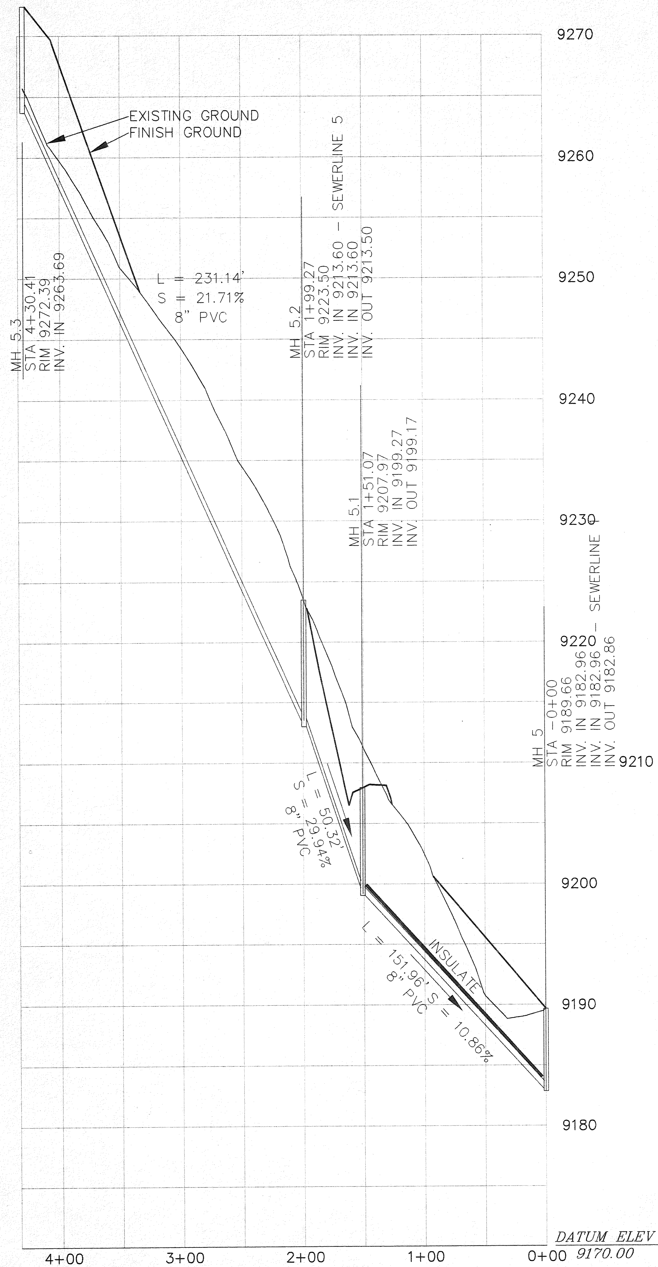
SEWER MAIN #4 SCALE: HORIZONTAL - 1" = 50' VERTICAL - 1" = 5'
