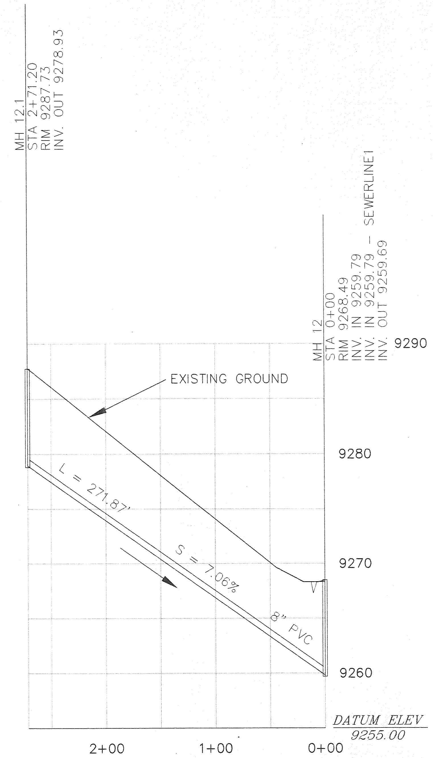
SEWER MAIN #6 SCALE: HORIZONTAL - 1" = 50' VERTICAL - 1" = 5'
