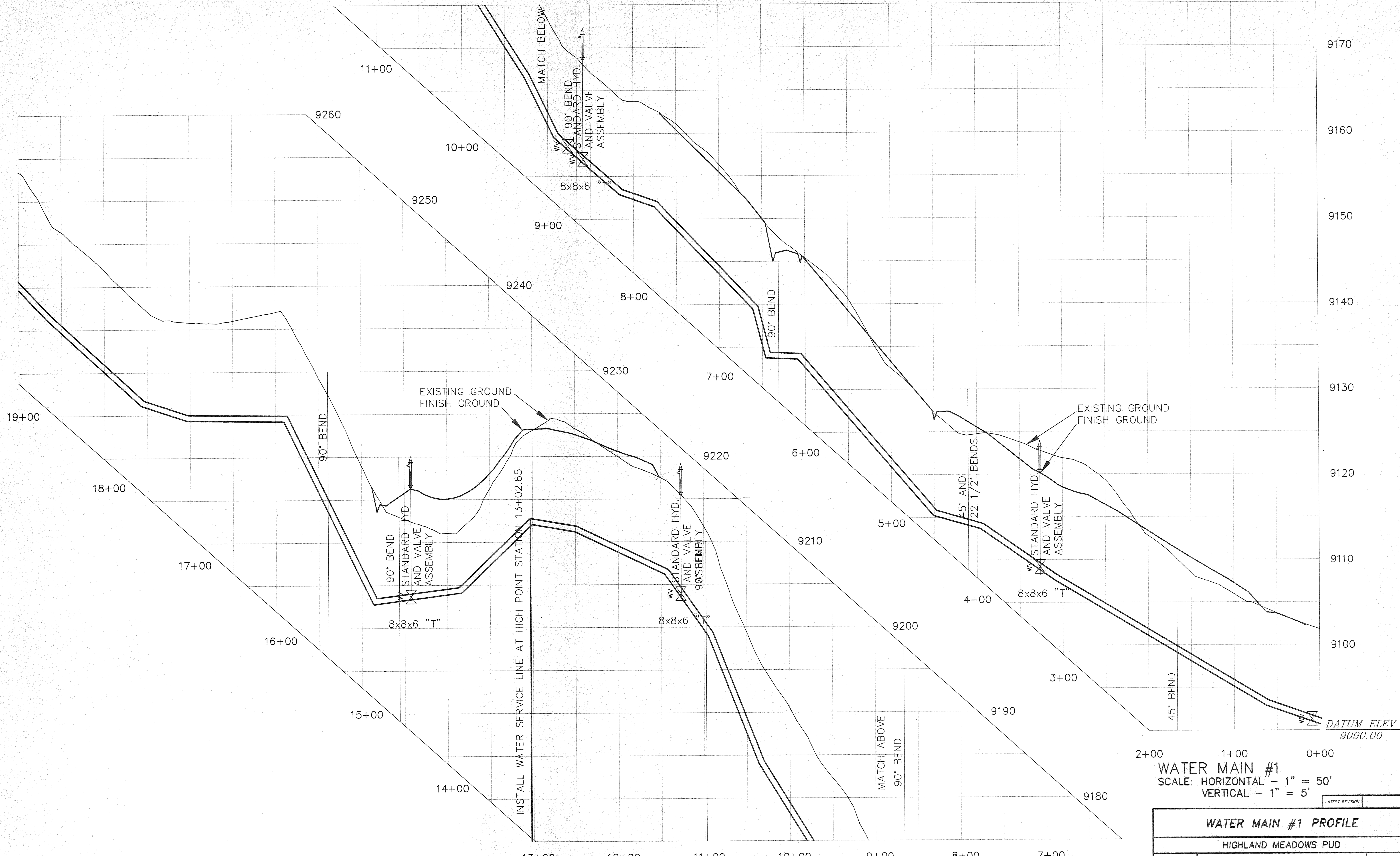
WATER MAIN #1 - 2 OF 5 SCALE: HORIZONTAL - 1" = 50' VERTICAL - 1" = 5'
